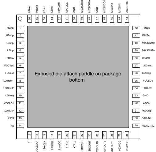
MT2122 Pin Diagram
